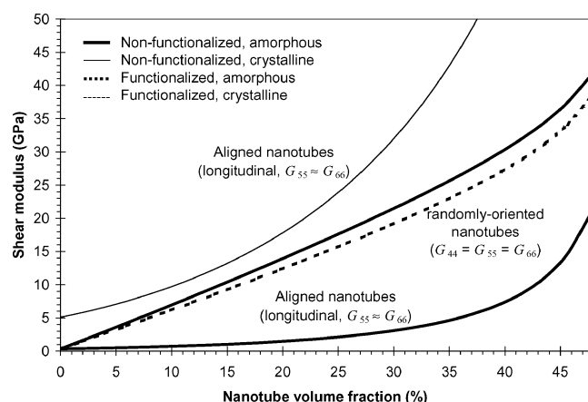
Fig. 9 Longitudinal shear moduli G_{55} and G_{66} of the composite systems vs nanotube volume fraction for a nanotube length of 400 nm.
