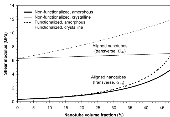
Fig. 10 Transverse shear moduli G_{44} of the composite systems vs nanotube volume fraction for a nanotube length of 400 nm.
